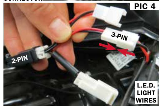
ACCESSORY CONNECTOR
